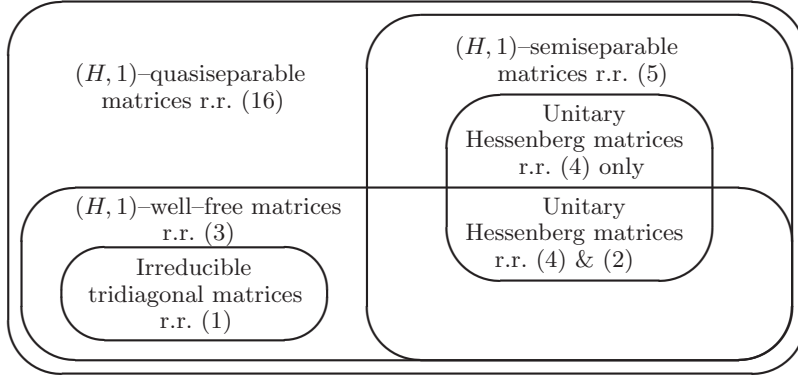
Fig. 1. Relations between subclasses of (H, 1) -quasiseparable matrices, from [BEGO08].
