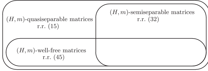
Fig. 3. Relations between subclasses of (H, m) -quasiseparable matrices.
