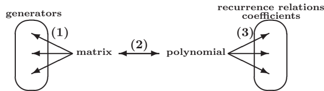
Fig. 4. Relations between subclasses of (H, m) -quasiseparable matrices and polynomials.
